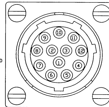
J6 PINOUT
